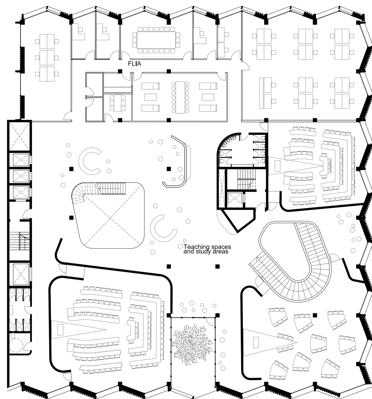
PLAN LEVEL 1 - 1:250
