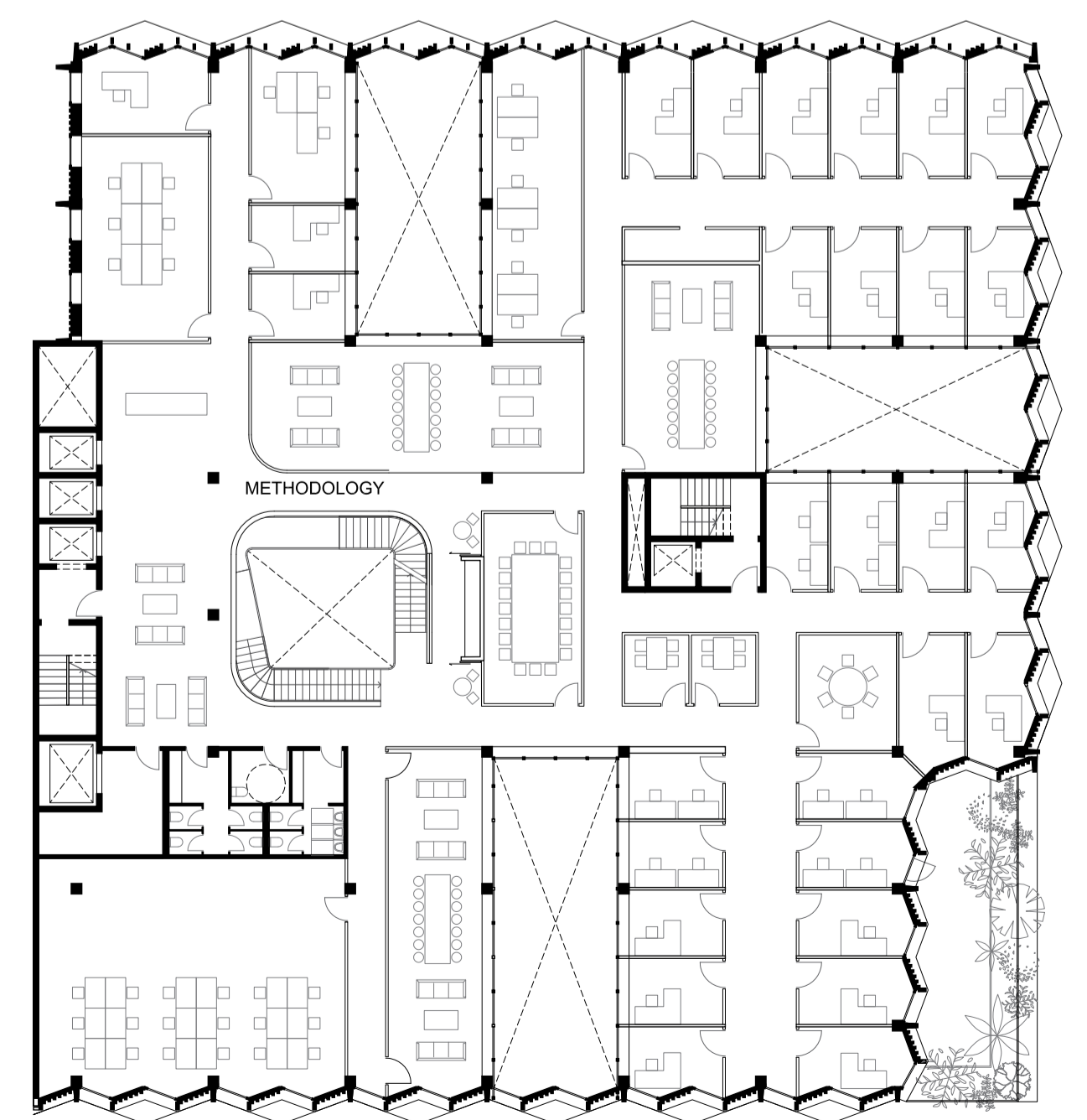
PLAN LEVEL 3 - 1:250
