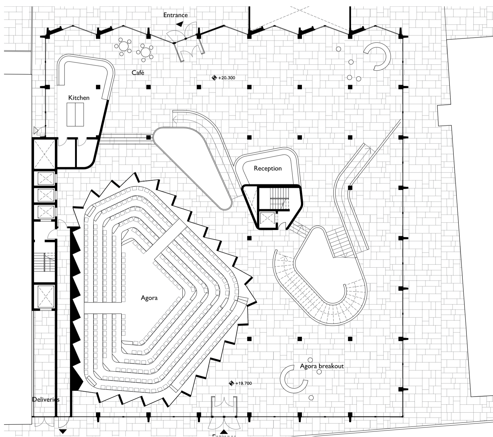
PLAN ENTRANCE LEVEL - 1:250
