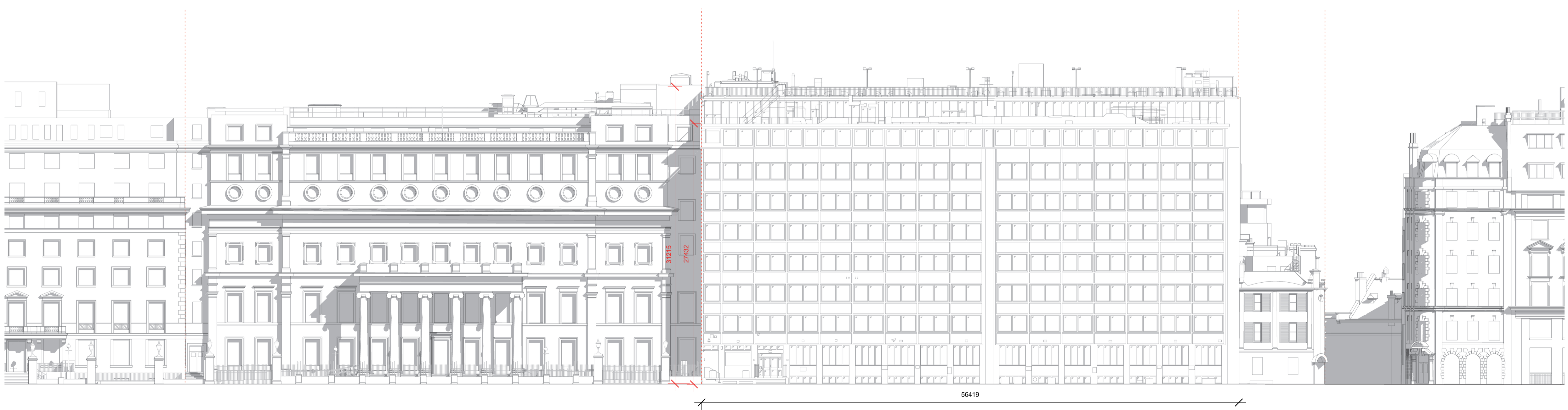
Existing North Elevation - Before | 1:250
