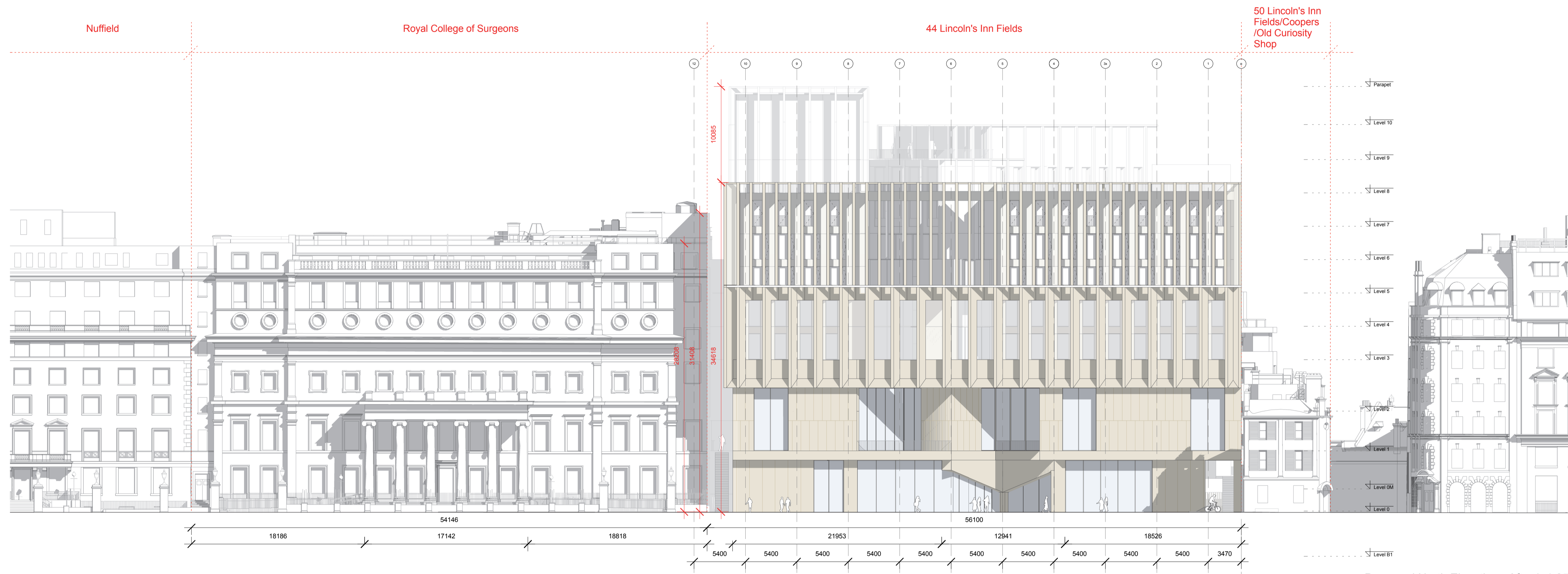
Proposed North Elevation - After | 1:250
