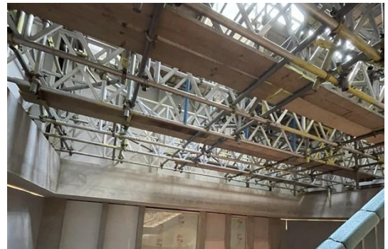
Crash deck system installed from L7 to L9
