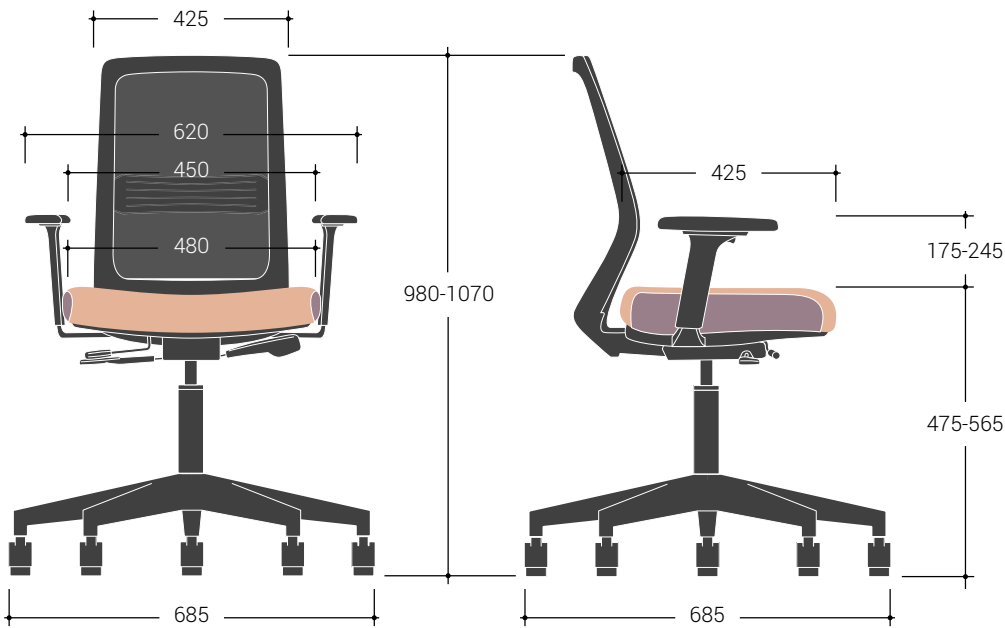
Task Chair VID/1D/PB Overall Dimensions: 1070h x 685w x 685d
