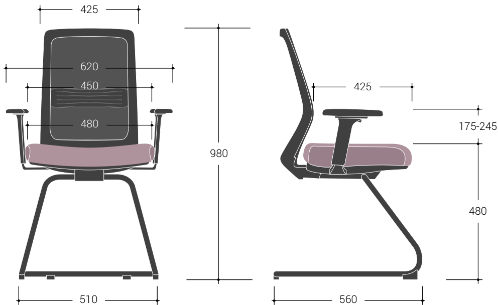
Cantilever Chair VIDC/1D Overall Dimensions: 980h x 620w x 560d
